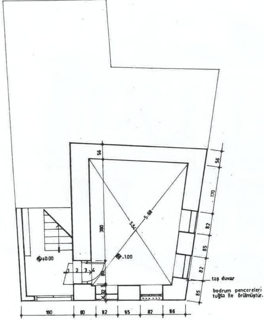
BODRUM KATI PLANI 1/50
